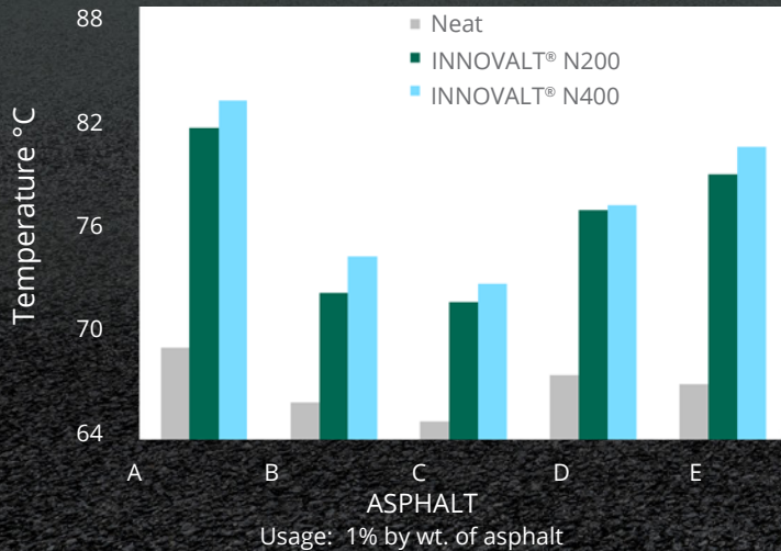
INNOVALT® PPA Impact on High Temperature Properties
