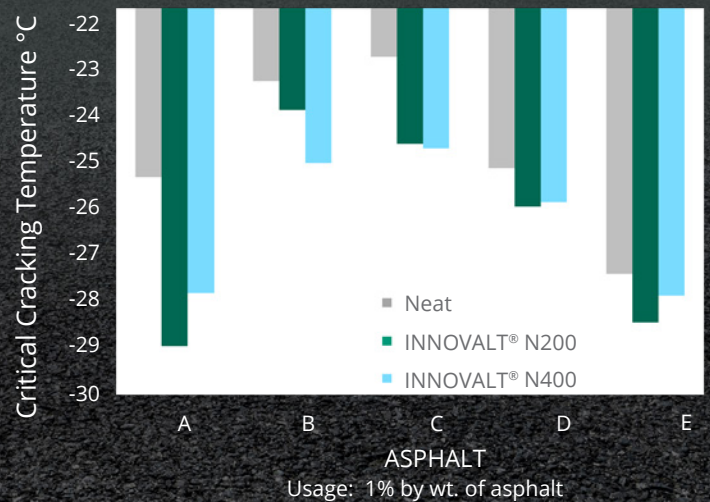
INNOVALT® PPA Impact on Low Temperature Properties
