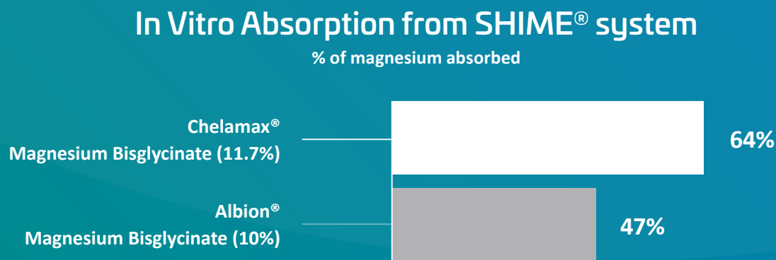
Figure 3. Comparison of Innophos Chelamax® Magnesium Bisglycinate versus Albion® Magnesium Bisglycinate using the SHIME® in vitro system.
