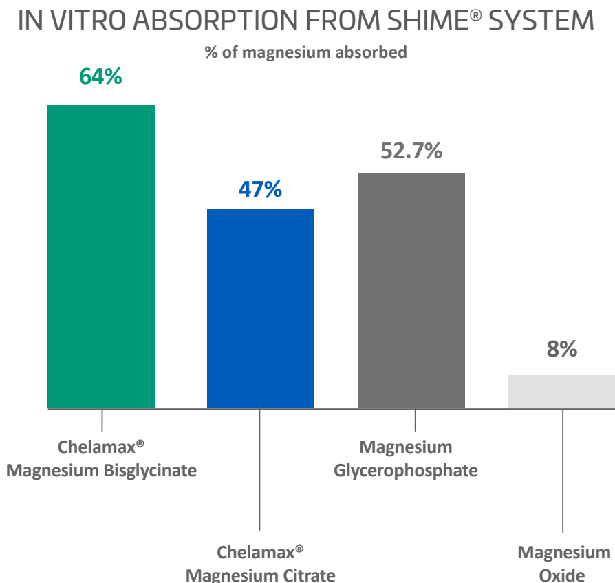
Figure 2. The percentage of magnesium absorbed by each sample in the ProDigest® SHIME® test system represents the final test point after 3h in the dialysis membrane.
