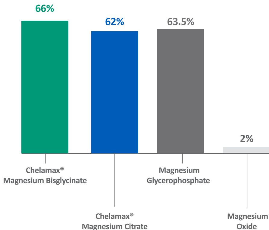
Figure 1. Magnesium oxide is poorly bioaccessible while the organically bound products remain soluble. The improved solubility allows for greater bioaccessibility in the small intestine where absorption occurs.
